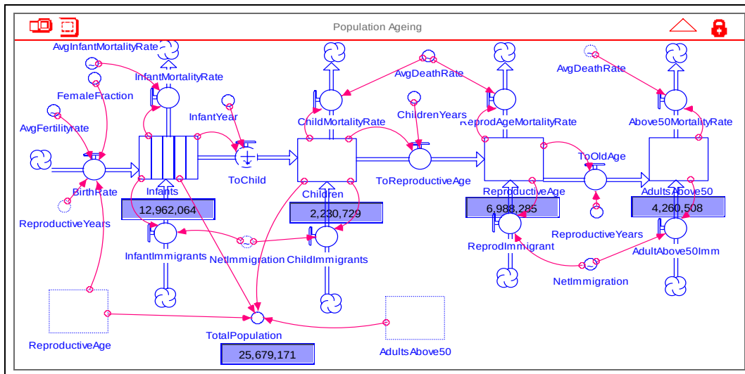
Figure 8 : Population Ageing Sector
